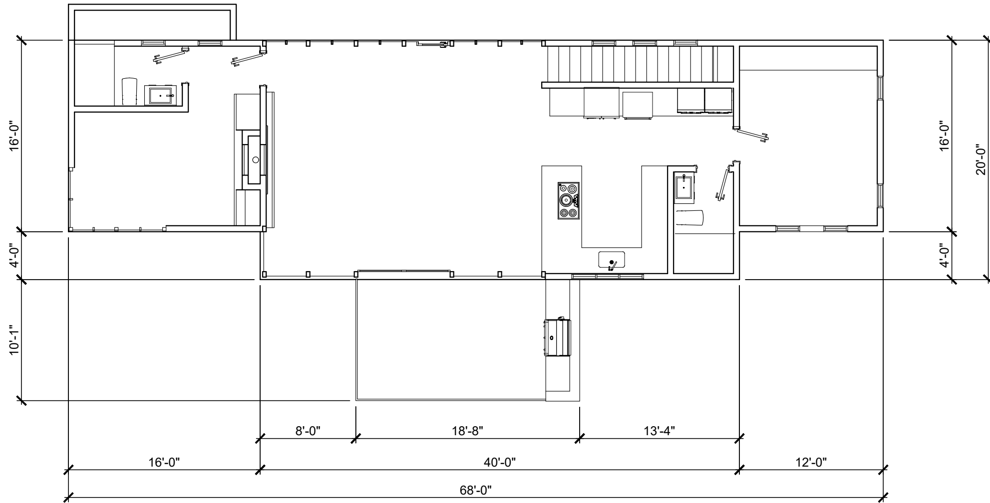
1st FLOOR PLAN 1248 SF
